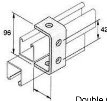
Double Channel C Brackets
