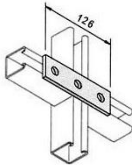
3 Hole Plate
