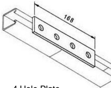
4 Hole Plate
