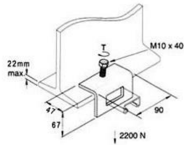
Window Brackets
