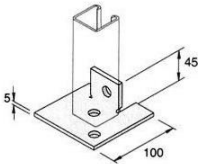
Single Channel Base Plate
