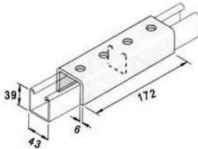
Extra Channel Coupler
