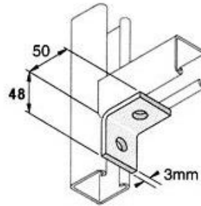
2 Hole Bracketry
