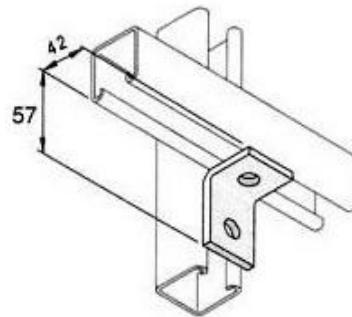
2 Hole Bracketry
