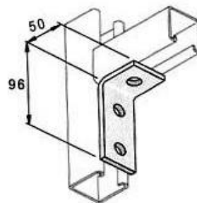
Angle Bracket 90°
