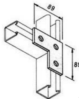
4 Hole Plate
