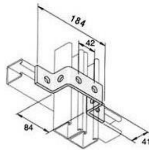
Double Channel Bracket
